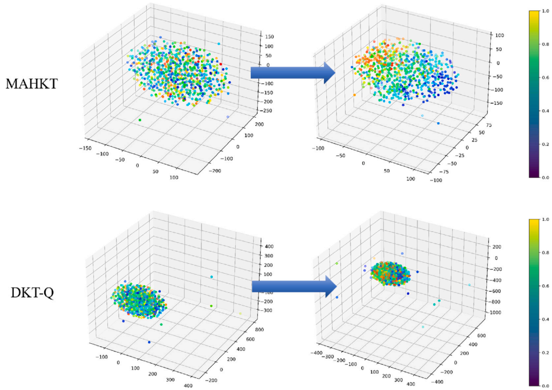
Fig. 4. Visualization of question embeddings in the JUNYI2015 dataset. The top image shows the clustering of the MAHKT model before and after training with heterogeneous graph embedding and knowledge propagation, whereas the bottom image shows the clustering for the DKT-Q model. The MAHKT model achieves better clustering.
