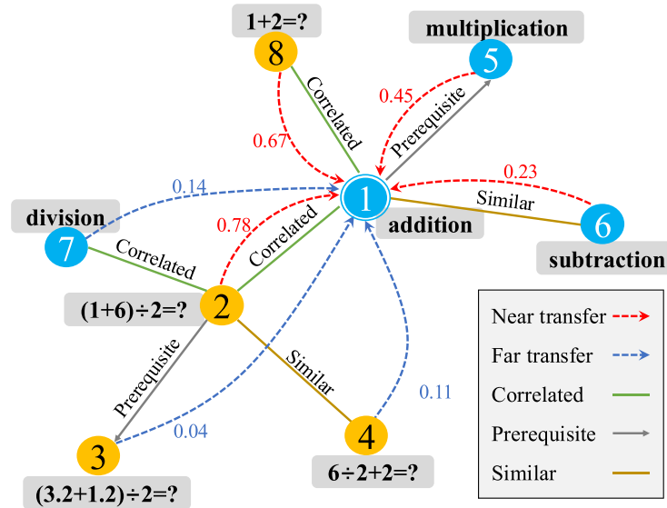
Fig. 5. Visualization of near and far transfer effects cases between concepts and questions in the JUNYI2015 dataset.
