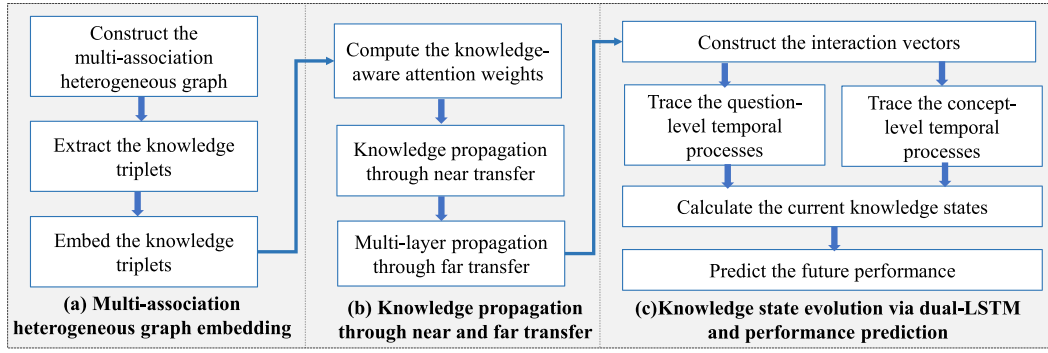
Fig. 2. The overview flowchart of the MAHKT method consists of three modules: (a) constructing a multi-association heterogeneous graph with five associations and extracting knowledge triples; (b) performing near- and far-transfer using knowledge-aware attention, aggregating neighboring knowledge, and propagating multi-layer representations to capture higher-order dependencies; and (c) evolving knowledge states with a dual-LSTM to trace learners' knowledge across questions and concepts, predicting future responses.
