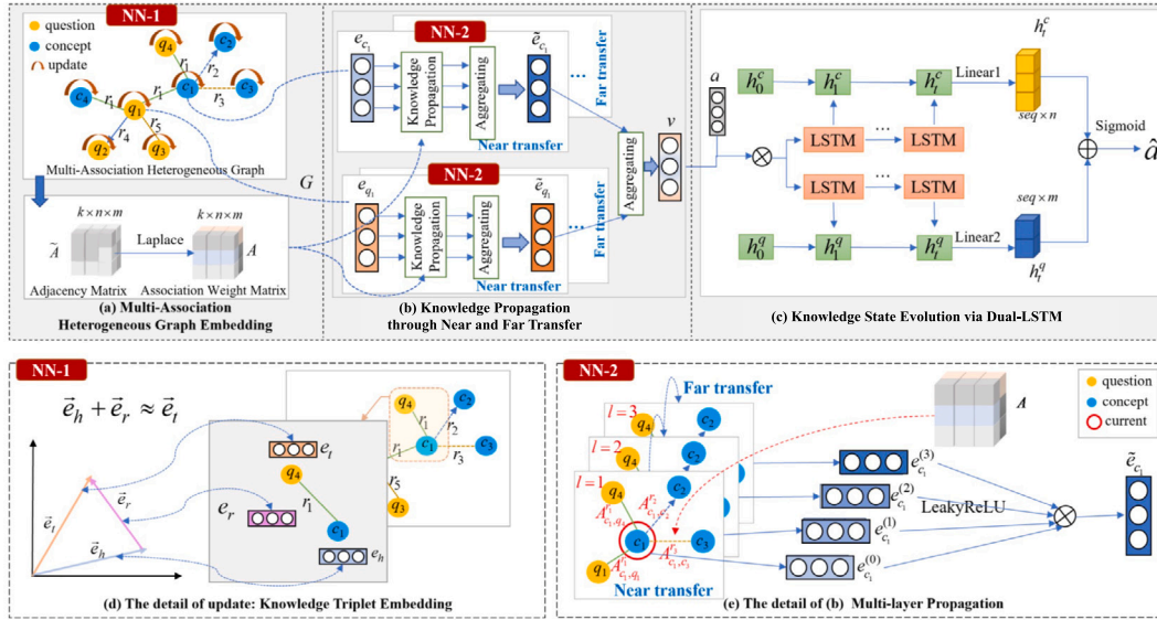
Fig. 3. The detailed overview of MAHKT framework. MAHKT consists of three primary modules: (a) Multi-Association Heterogeneous Graph Embedding, (b) Knowledge Propagation through Near and Far Transfer, and (c) Knowledge State Evolution via Dual-LSTM and Performance Prediction. The specific processes for the first two modules are detailed as NN-1 and NN-2, shown in parts (d) and (e).
